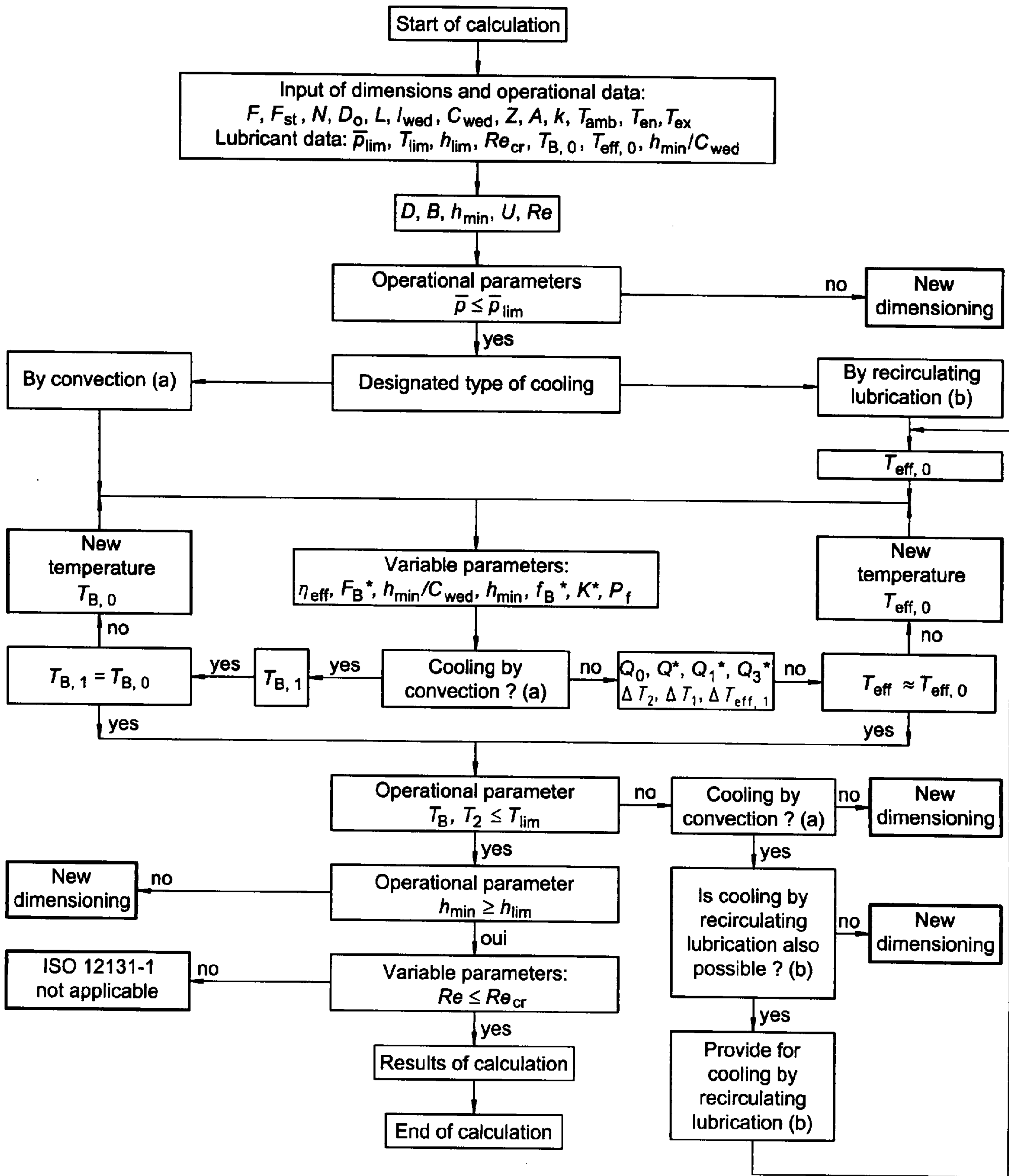
Figure 2 — Scheme of calculation (flow chart)
